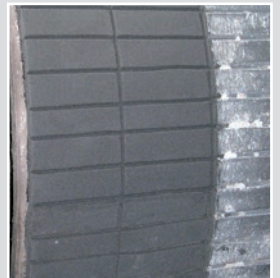
Application, compression and texturing of the ceramic compound
